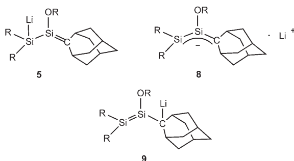
Scheme 4. Possible structural isomers of 5 , 8 , and 9 ; R = SiMe 2 Bu 2 .
