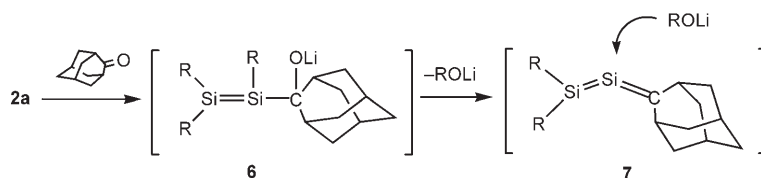
Scheme 3. Reaction pathway to form 5 by the reaction of disilenyllithium 2a with adamantanone; R = SiMe 2 Bu 2 .
