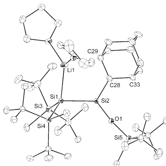
Figure 1. Crystal structure of 5 (ORTEP plot; thermal ellipsoids are shown at the 30% probability; hydrogen atoms are omitted). Selected bond lengths [Å] and angles [°]: Si1–Si2 2.3246(6), Si1–Si3 2.3855(6), Si1–Si4 2.3734(6), Si1–Li1 2.685(3), Si2–C28 1.7431(17), Si2–O1 1.6560(12); O1–Si2–C28 112.50(7), O1–Si2–Si1 127.70(5), C28–Si2–Si1 119.77(6), C29–C28–C33 109.87(14), C29–C28–Si2 126.60(13), C33–C28–Si2 123.33(13), Si2–Si1–Si4 109.98(2), Si2–Si1–Si3 108.74(2), Si3–Si1–Si4 118.42(2), Si5–O1–Si2 171.47(8), Si2–Si1–Li1 85.97(8), Si3–Si1–Li1 131.13(7), Si4–Si1–Li1 97.56(7).
